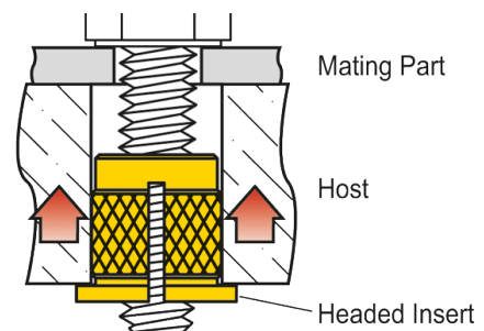
Figure 3: In high load applications, consider locating the head of the insert opposite the load to increase pull-out strength. Tapered inserts should not be used in pull-through applications
