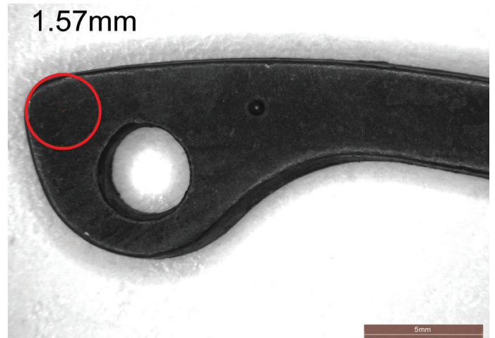
Detail of the lug of a retaining ring blanked by steel strip (zoom: 6.3X). Radius of 1.57mm on the external side of the ring
