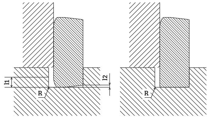
Figure 2: How both cross sections sit into the groove
