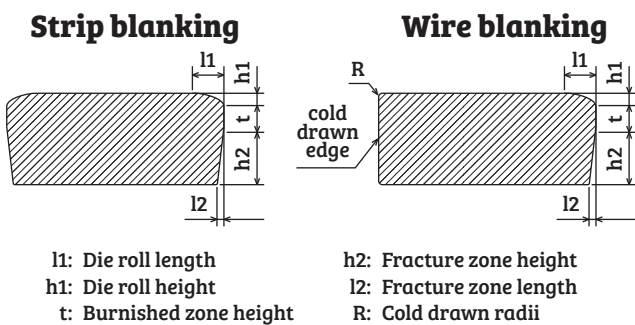
Figure 1: Each production technology generates a specific cross section of the retaining ring
