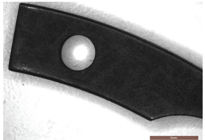
Detail of the lug of a retaining ring cut by wire (zoom: 6.3X). Sharp-edged shape on the external side of the ring
